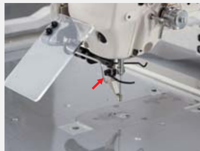
Needle cooler
